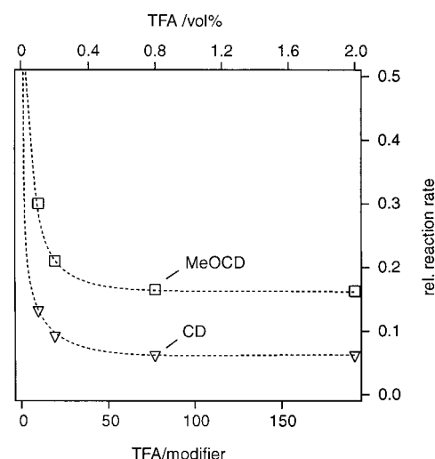
Figure 3. Hydrogenation of 1 in the presence of CD or MeOCD: comparison of the reaction rates related to the rates in pure toluene.
