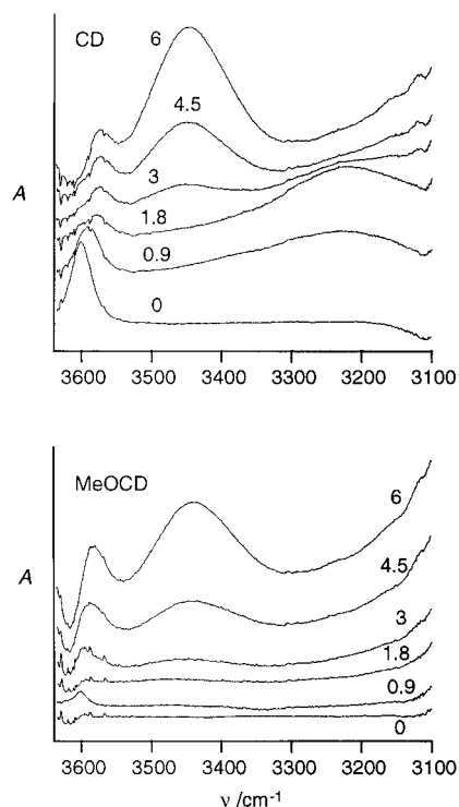
Figure 5. \nu(\text{OH}) region of the IR spectra of solutions of CD and MeOCD in \text{CH}_2\text{Cl}_2 containing different amounts of TFA (TFA/modifier molar ratio between 0 and 6). Modifier concentrations are higher by a factor of 2.5 compared to the standard reaction procedure. Spectra are offset.
