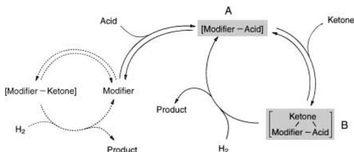
Figure 8. Three-step reaction mechanism proposed for the enantioselective hydrogenation of trifluoromethyl ketones in the presence of carboxylic acids. The presently accepted two-step reaction mechanism (valid in the absence of carboxylic acids) is indicated by dashed lines.
