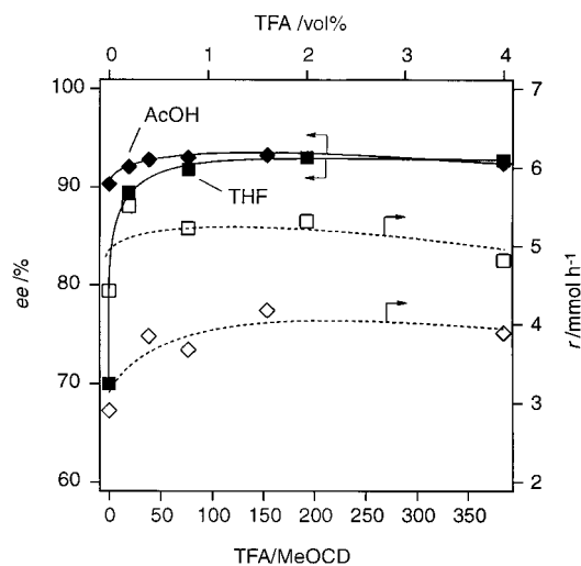
Figure 4. Hydrogenation of 1 using MeOCD as chiral modifier: changes in ee and reaction rate ( r ) upon addition of TFA to THF or AcOH. Open symbols: reaction rate; closed symbols: ee .
