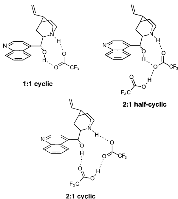
Figure 7. Structures of TFA-CD complexes (complex A in Figure 8) formed in solution at low TFA concentration.
