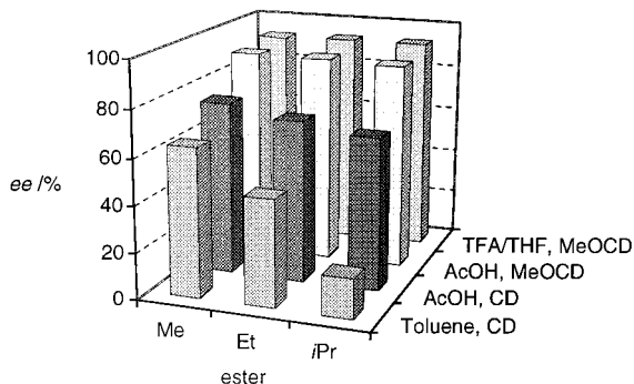
Figure 10. Enantioselectivities obtained in the hydrogenation of methyl-, ethyl- and isopropyl-4,4,4-trifluoroacetate in the presence or absence of acid.
