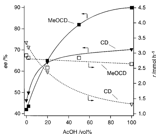
Figure 1. Hydrogenation of 1 in AcOH/toluene mixtures using CD or MeOCD as chiral modifiers. Open symbols: reaction rate ( r ); closed symbols: ee .
