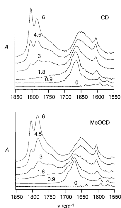
Figure 6. \nu(\text{C}=\text{O}) region of the IR spectra of solutions of CD and MeOCD in \text{CH}_2\text{Cl}_2 containing different amounts of TFA (TFA/modifier molar ratio between 0 and 6). Modifier concentrations are higher by a factor of 2.5 compared to the standard reaction procedure. Spectra are offset.
