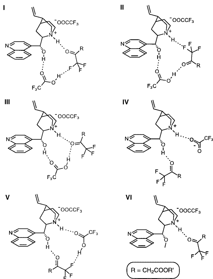
Figure 9. Possible structures of the reactant–modifier–carboxylic acid complex (complex B in Figure 8) responsible for enantio-discrimination (note that the interaction with the metal surface is not included).
