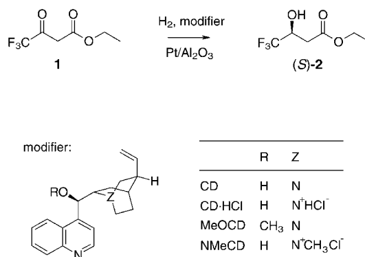
Scheme 1. Hydrogenation of ethyl-4,4,4-trifluoroacetoacetate ( 1 ) over chiral modified Pt/Al 2 O 3 .
