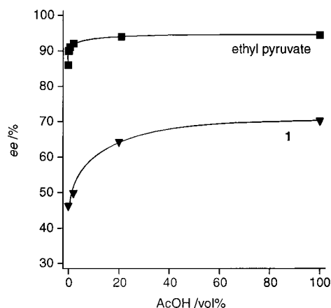
Figure 11. Comparison of the enantioselectivities in the hydrogenation of 1 and ethyl pyruvate in AcOH/toluene mixtures, using cinchonidine as chiral modifier.
