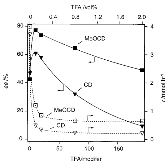
Figure 2. Hydrogenation of 1 in toluene using CD and MeOCD as chiral modifiers: changes in ee and reaction rate ( r ) upon addition of TFA. Open symbols: reaction rate; closed symbols: ee .
